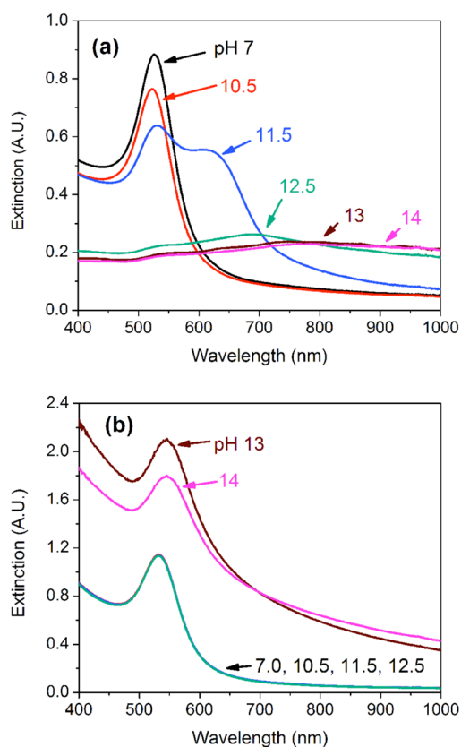
Figure 4. Extinction spectra of colloidal (a) SiO 2 -coated Au nanoparticles and (b) SnO 2 -coated Au nanoparticle solutions at various pH values. The spectra were recorded approximately 1 h after the solution pH values were adjusted using 0.1 M NaOH.
