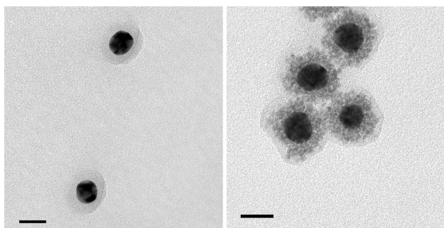
Figure 1. TEM images of (left) SiO 2 -coated gold nanoparticles and (right) SnO 2 -coated gold nanoparticles. The scale bars are 20 nm.
