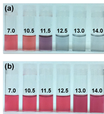
Figure 3. Photographs of colloidal (a) SiO 2 -coated Au nanoparticle and (b) SnO 2 -coated Au nanoparticle solutions at various pH values. The photographs were taken approximately 1 h after the solution pH values were adjusted using 0.1 M NaOH. The loss of dispersion for the SiO 2 -coated Au nanoparticles at high pH, however, occurred immediately upon adjustment of the pH.
