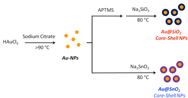
Scheme 1. Synthesis of SiO 2 -Coated Au Nanoparticles and SnO 2 -Coated Au Nanoparticles
